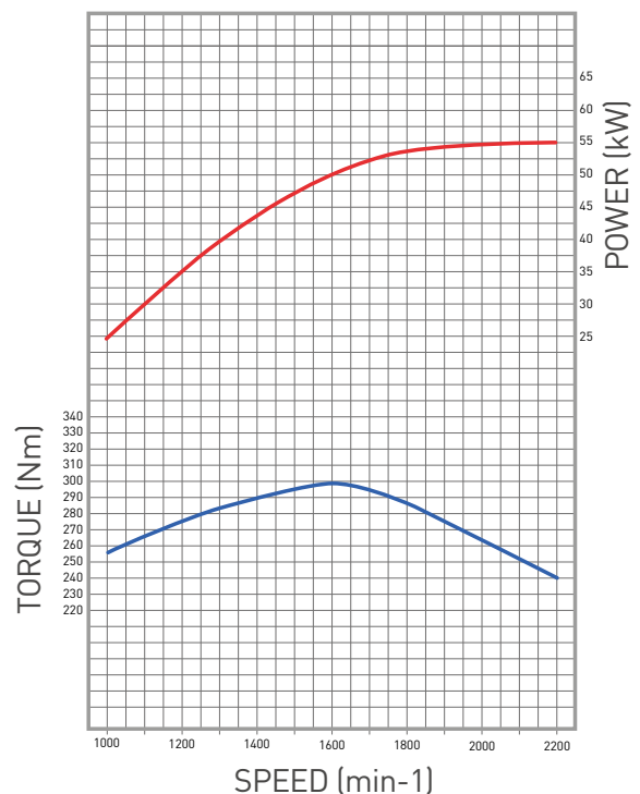
TCD 2.9 L4 ENGINE
